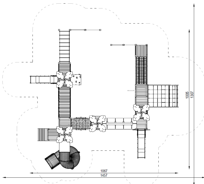
Top view with falling area
